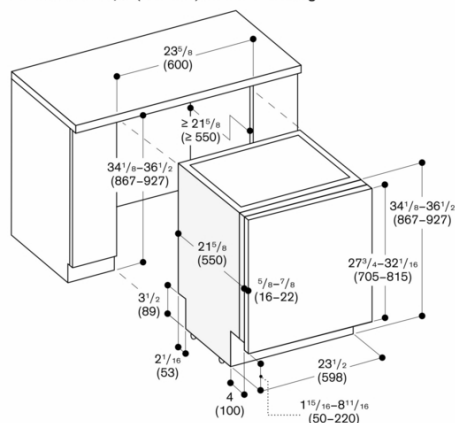
Dishwasher 34 1 / 8 " (867 mm) with flexible hinge
