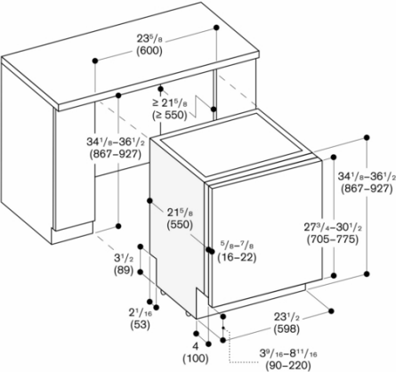
Dishwasher 34 1/8" (867 mm)
