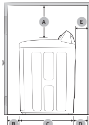
Side view - closet or confined area
