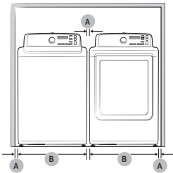
Recessed area
