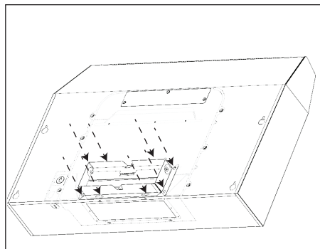
5. Secure 3-1/4" x 10" starting collar with damper to the duct opening using (8) M4x8 screws.
