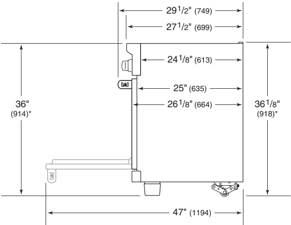
30" / 36" RANGE SIDE VIEW
