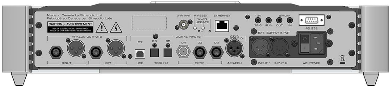
Figure 2: 780D Rear panel
