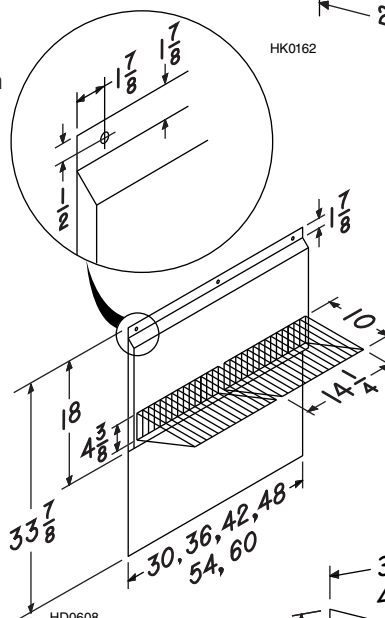
RMP Series Backsplash (Optional)
