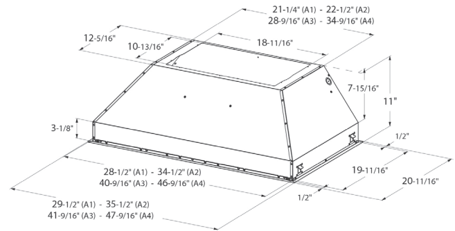
Overall 19" width
