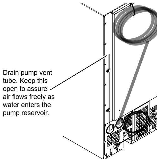
Figure 14: Location of vent tube.
