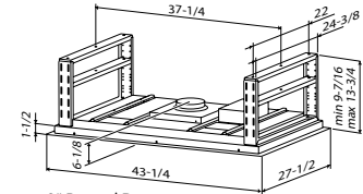
8" Round Duct
