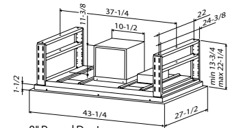
8" Round Duct
