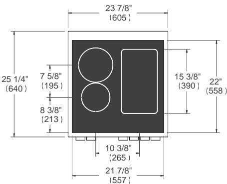
WORKTOP DETAILS
