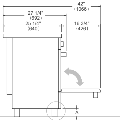
WORKTOP DETAILS
