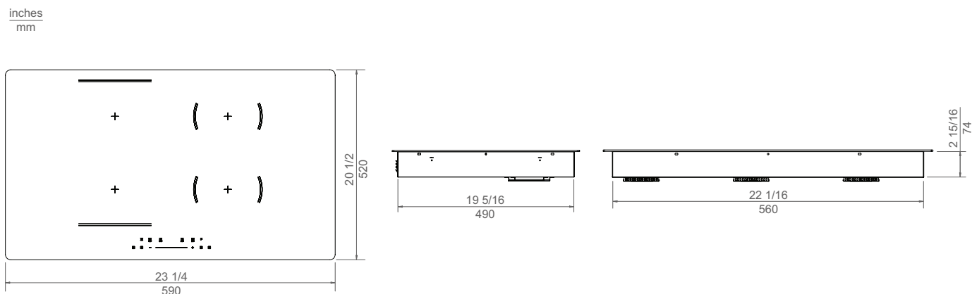
TOP VIEW
