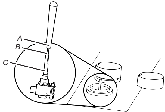
A. 3/32" (2.0 mm)—#0 flat-blade screwdriver (shaft must be a minimum of 2 1/2" [6.4 cm] long) B. Control knob stem opening C. Adjustment screw location
