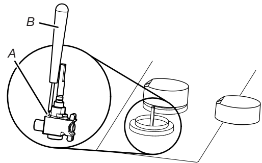
A. Adjustment screw location B. 3/32" (2.0 mm)—#0 flat-blade screwdriver (shaft must be a minimum of 2 1/2" [6.4 cm] long)
